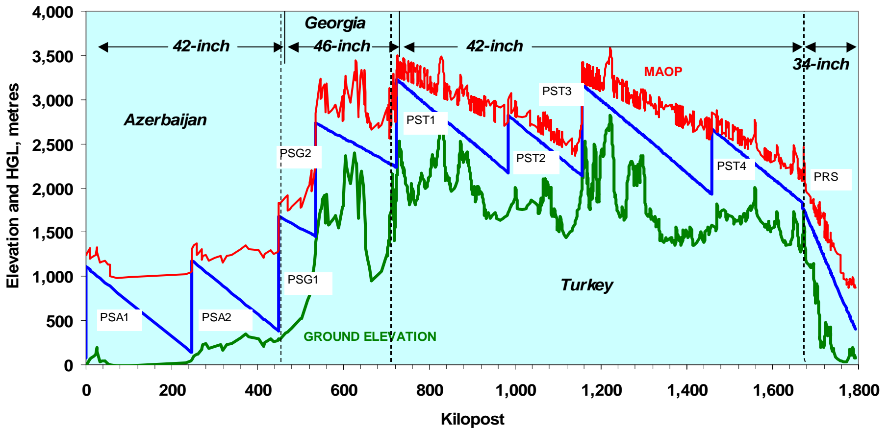
Hydraulic Gradient plotted against Ground Elevation and MAOP BTC Pipeline Case C7 @ Design Flowrate 50 Mta
